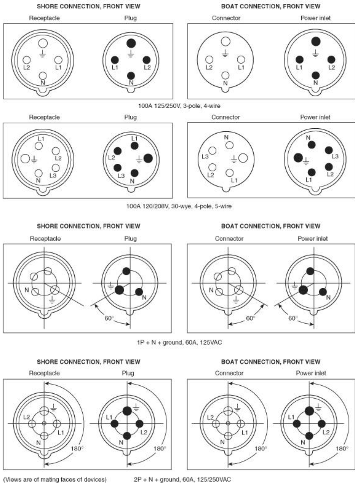
FIGURE 5.12.4 Safety Pin-and-Sleeve Configurations, Either 60 Amperes or 100 Amperes.
