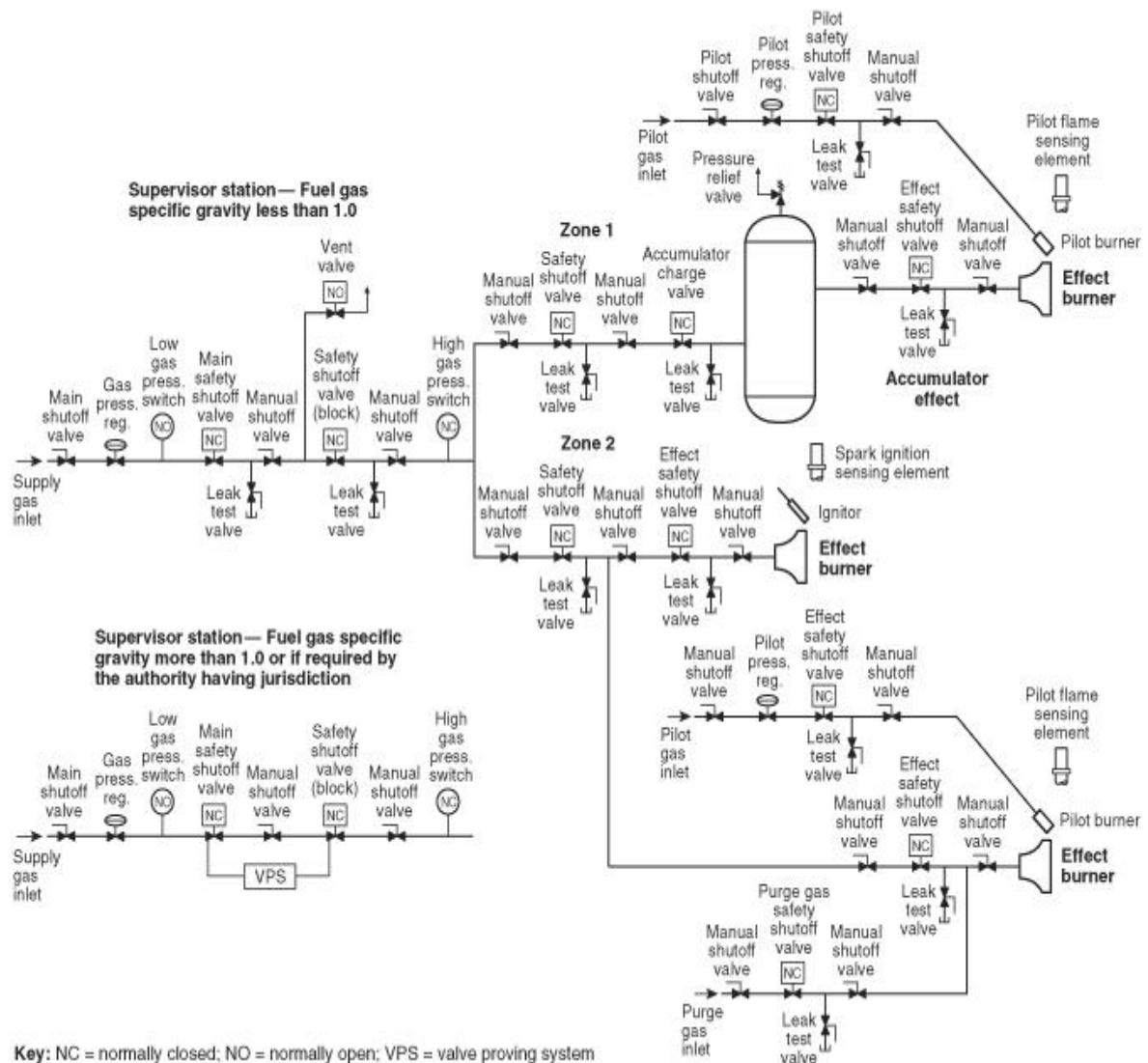
FIGURE A.9.3.2.4.1(3) Example of Various Flame Effect Control and Piping Components.
