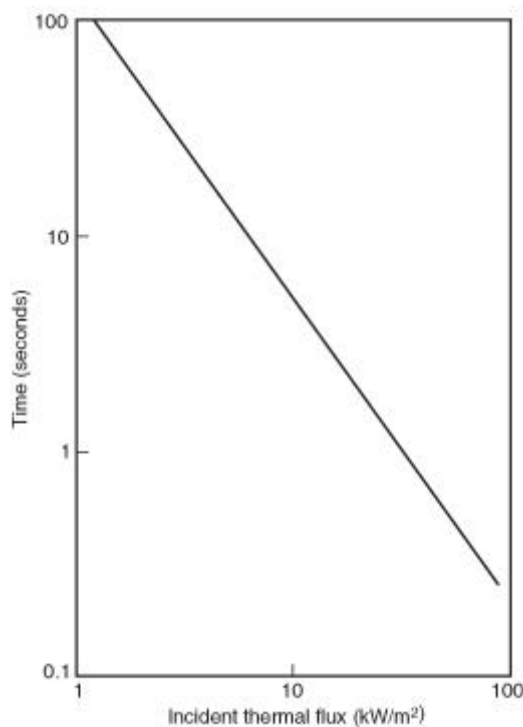
FIGURE A.7.1 Time Required for Pain Due to Exposure to Thermal Radiation.
